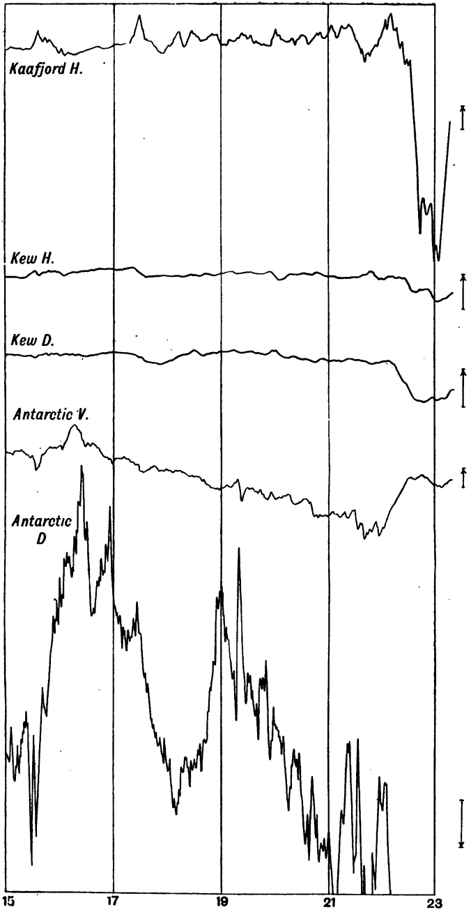
FIG. 31.—ARCTIC-KEW-ANTARCTIC CURVES.
